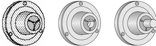
5C taper nose spindle illustrated.
